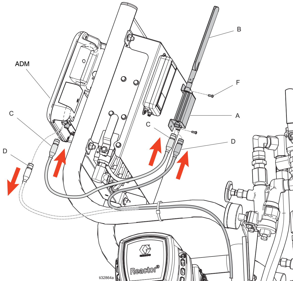
FIG. 1: Typical Reactor App Cell Module Installation
